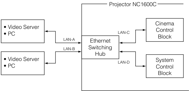
Internal Configuration Diagram of LAN Port
