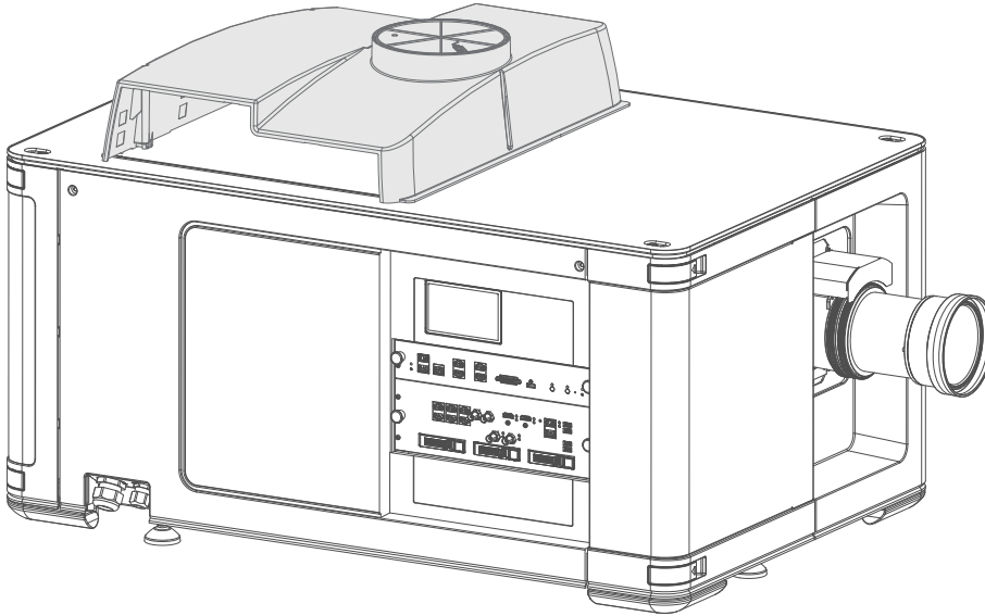
Image 2–10 Projector with exhaust adapter mounted
