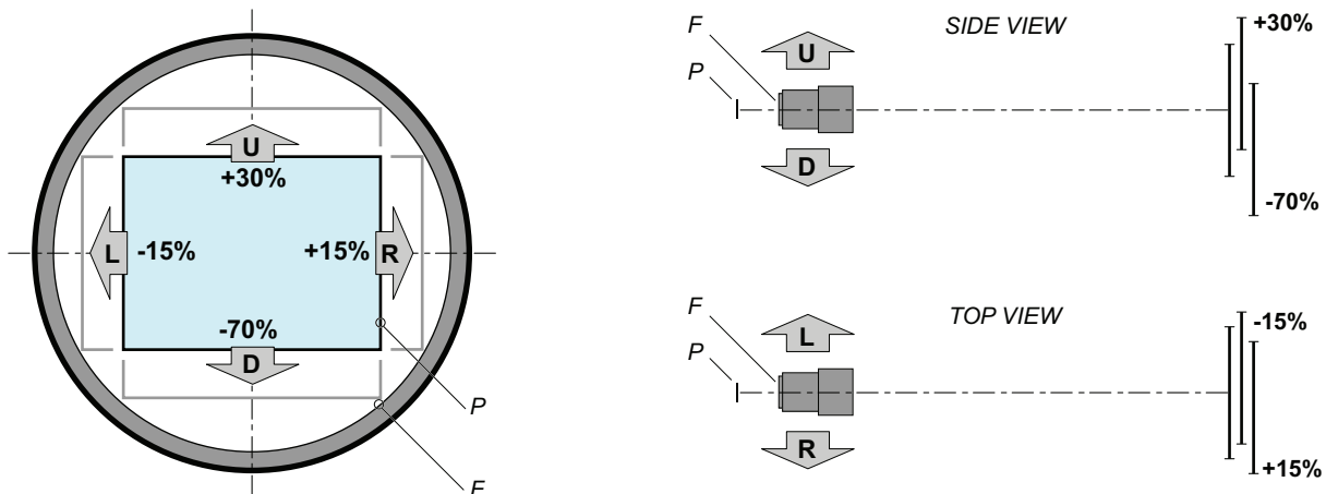
Image 5–9 Shift range for an SP2K-C projector with C-Lens holder
