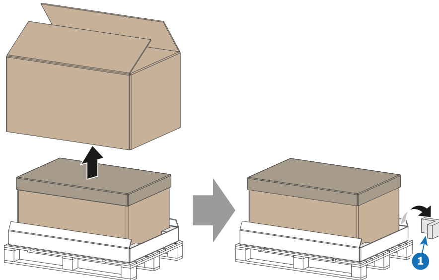
Image 2-3 Removing the outer cardbox and the four foam corner pieces
