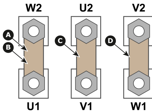
Image 4–9 Δ configuration
