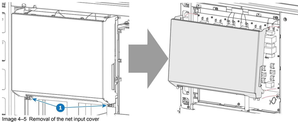
Image 4–5 Removal of the net input cover
