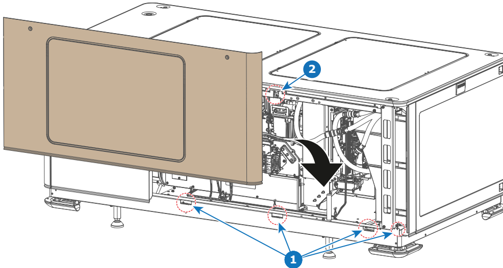
Image 12–12 Mounting the side cover
