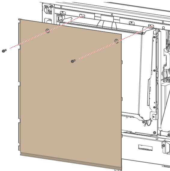
Image 12-18 Removal of the mains side cover
