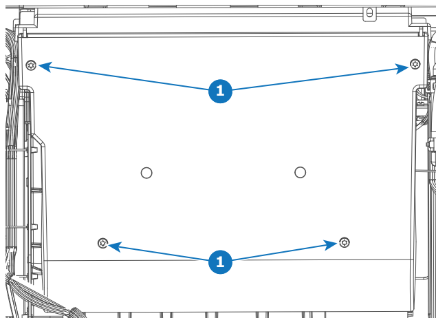
Image 10-1 Sealed cover fixation
