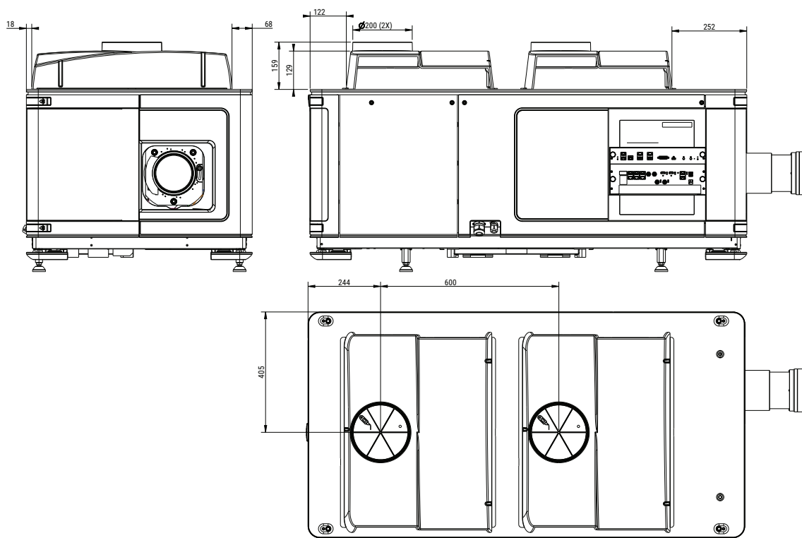
Dimensions of the projector with the exhaust adapters
