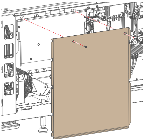
Image 12-6 Removal of the mains side cover
