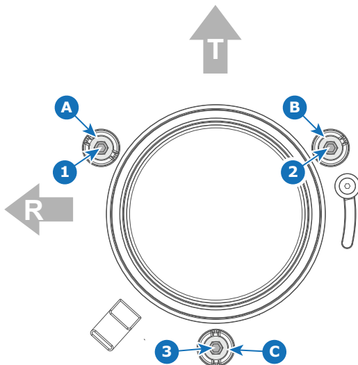
Image 5–14 Scheimpflug adjustments points on Lens holder - Projector front view. (Shape of the lens may vary with the model)
