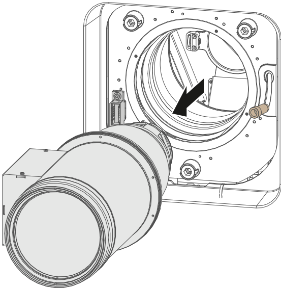
Image 5–7 Lens removal
