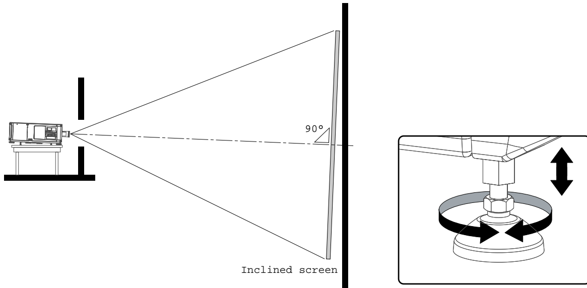
Image 4—4 Projector tilting
