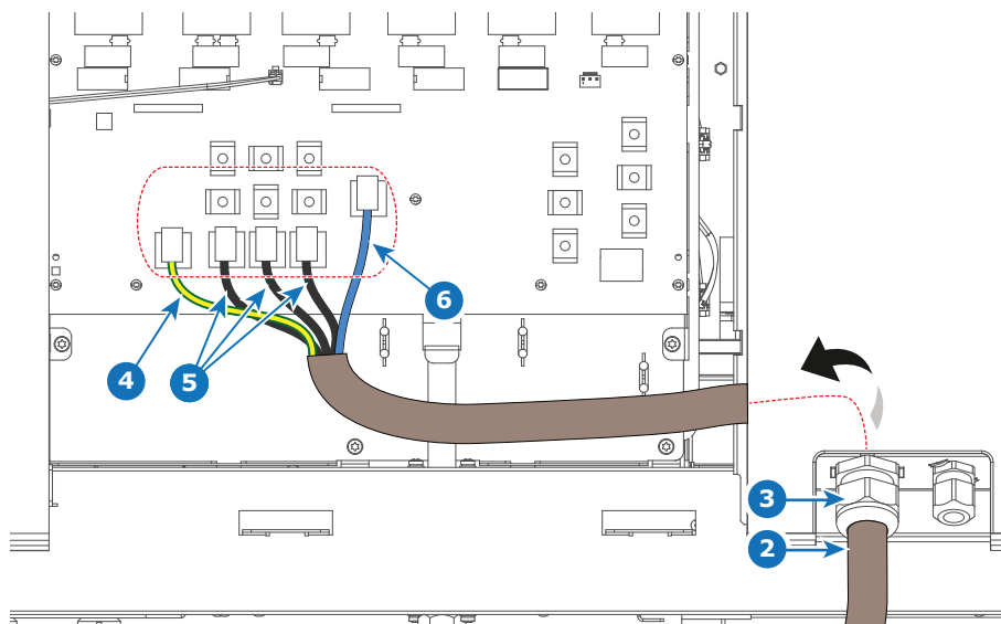
Image 4-11 Example of the power wiring
