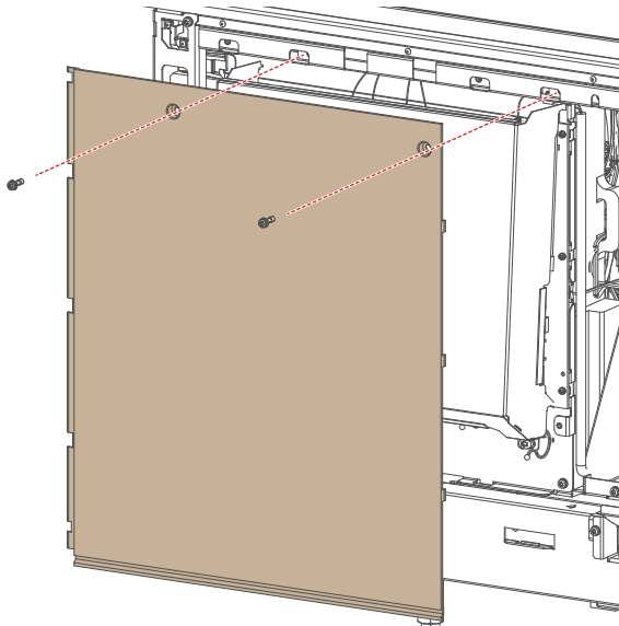
Image 12-3 Removal of the mains side cover
