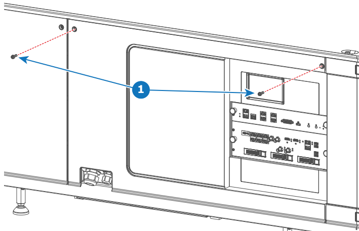
Image 12-17 Tightening the screws of the side cover
