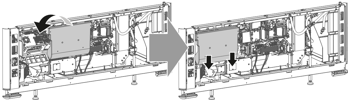
Image 10-5 Sealed compartment side cover, mount
