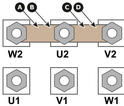
Image 4–8 Y configuration
