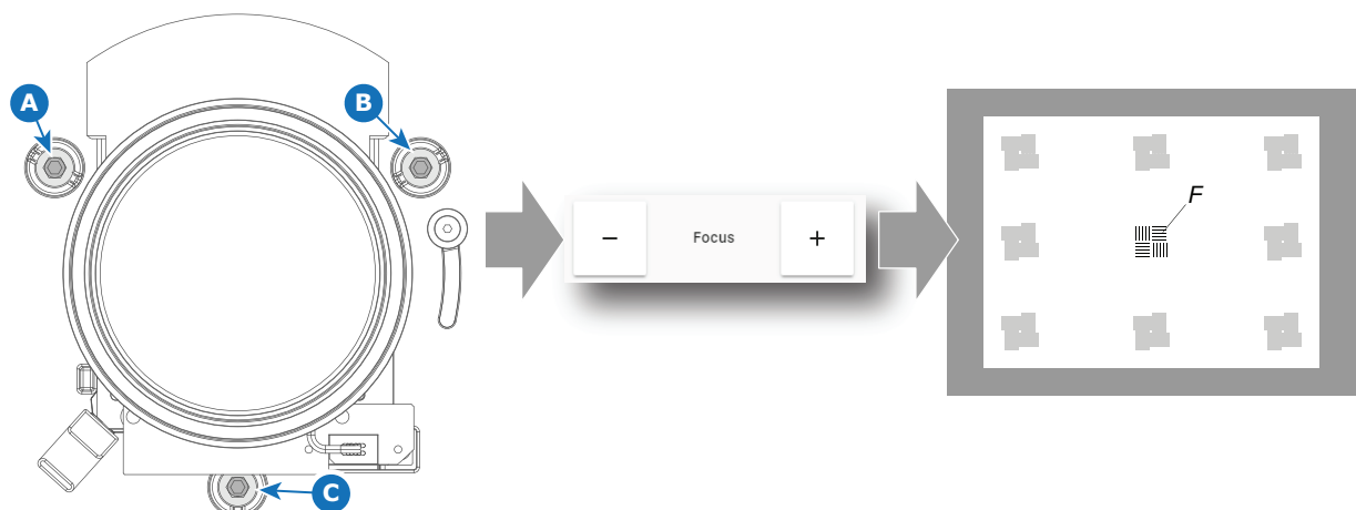
Image 5-16 Center focusing
