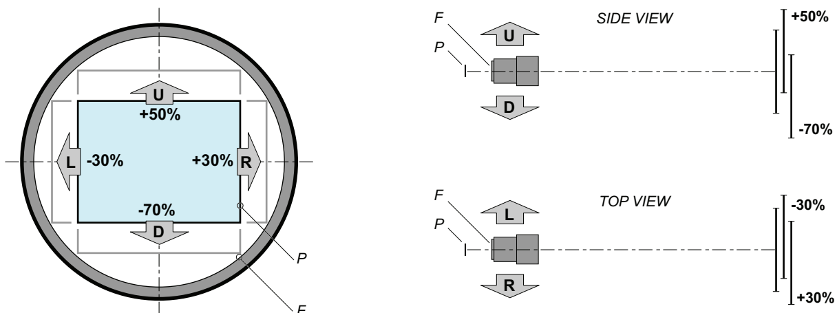
Image 5–9 Shift range for an SP4K-B projector
