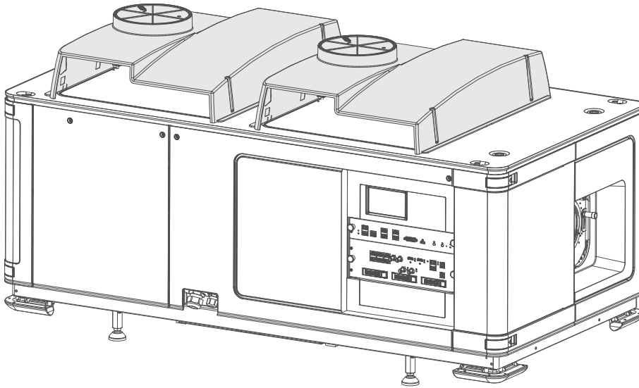
Image 2–15 SP4K-B projector with both exhaust adapters mounted
