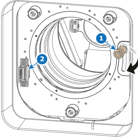
Image 5–2 Lens installation, preparing the lens holder
