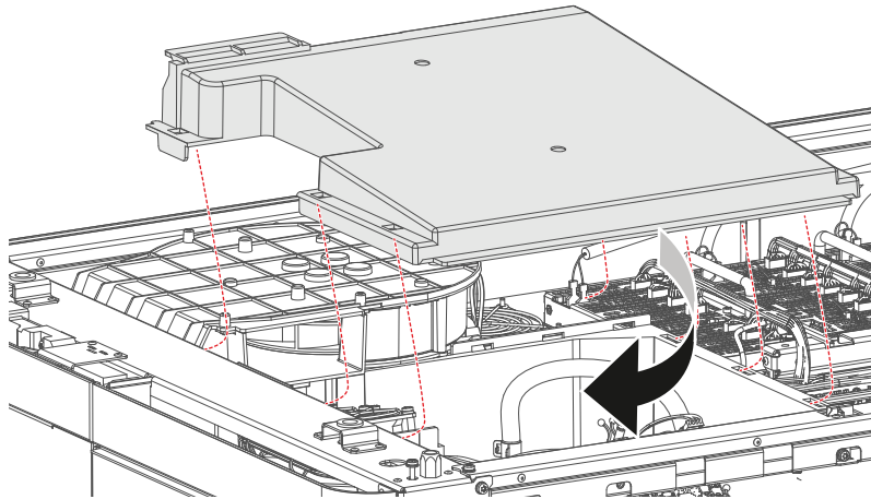
Image 10-4 Sealed top cover, mount
