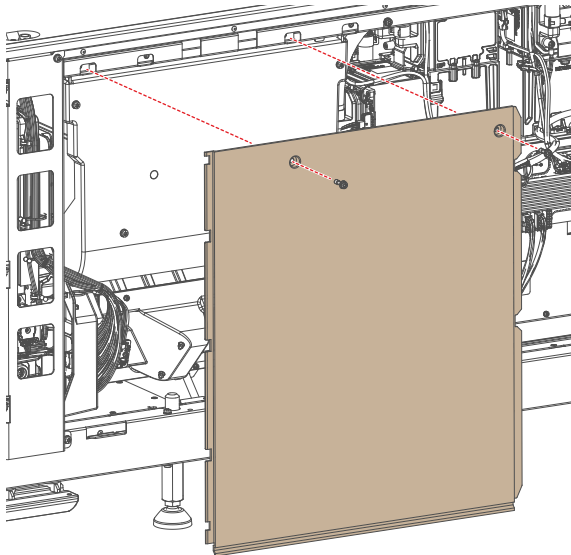
Image 12-14 Removal of the mains side cover
