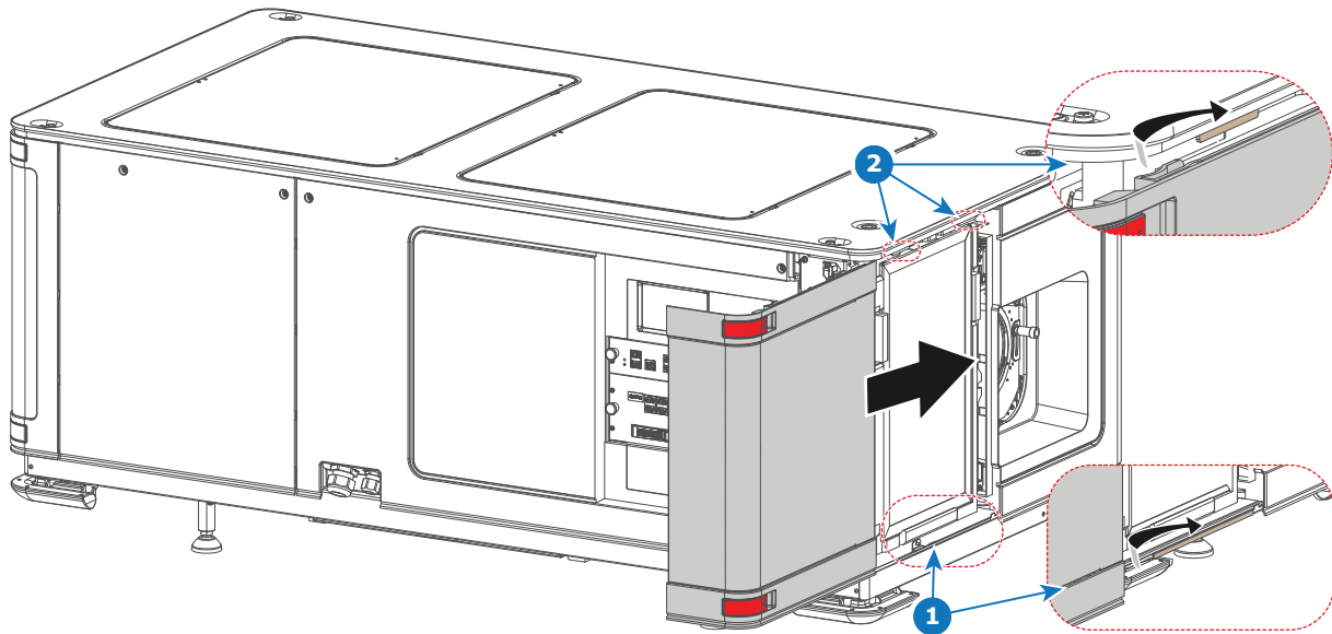
Image 12-20 Sliding in the front cover
