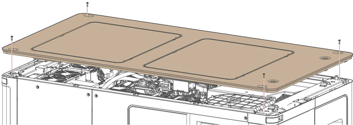
Image 12-11 Mounting the top cover
