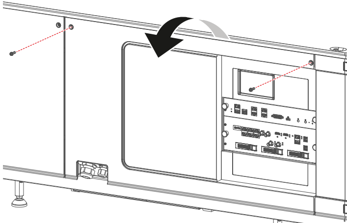
Image 12-4 Removing the screws of the right side cover
