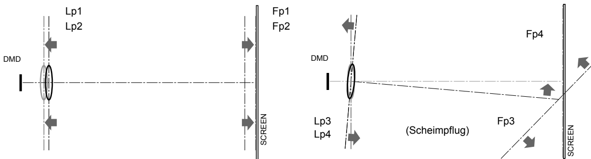
Image 5–13 Scheimpflug principle
