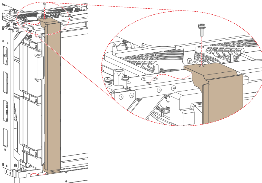
Image 12-9 Removing the small rear cover.
