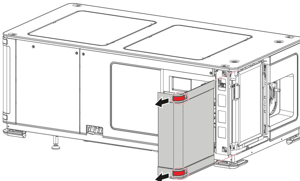
Image 12-1 Sliding the front cover away from the projector
