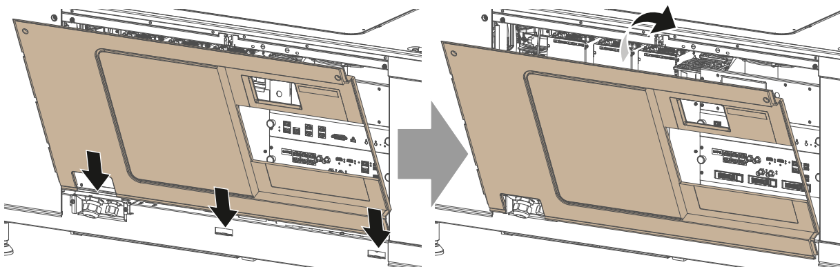
Image 12-16 Mounting the side cover
