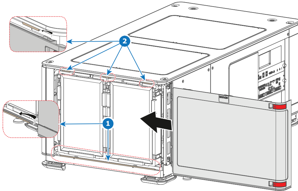
Image 12-19 Sliding in the rear cover
